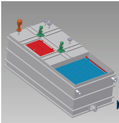
Compact physico-chemical station combining a coagulation tank, a flocculation tank and a lamellar decanter.
